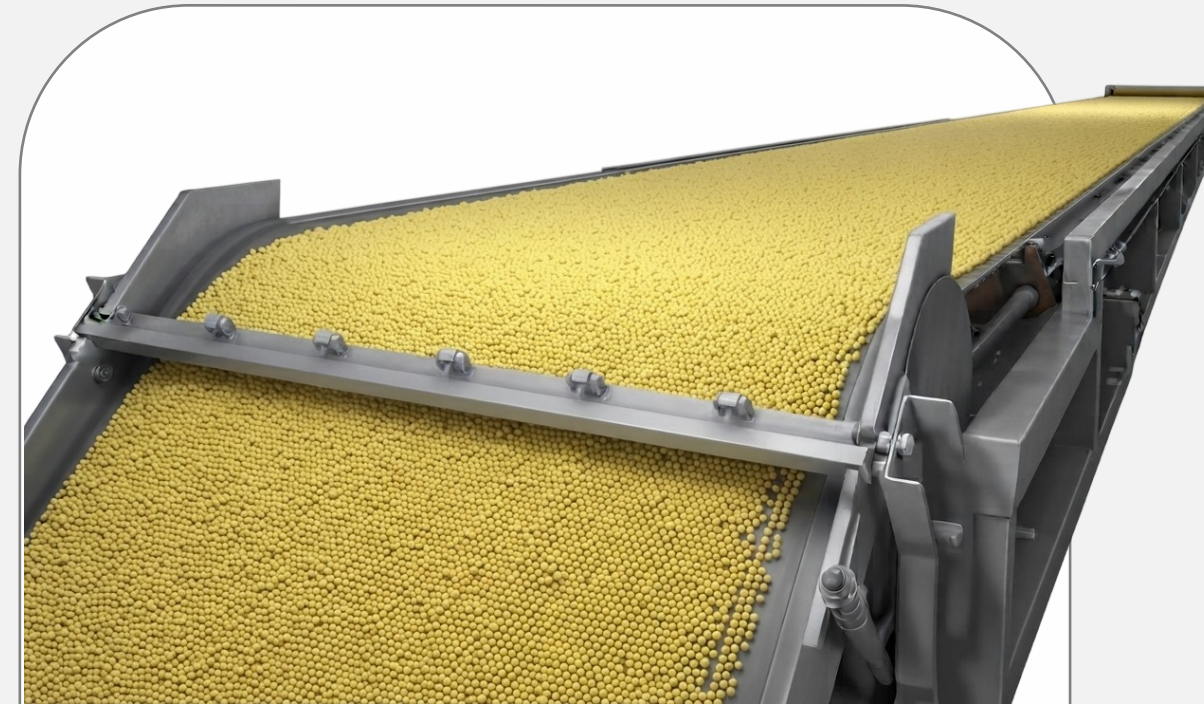
Belt Conveyor
