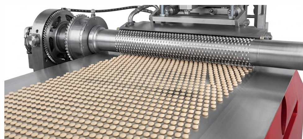
Granulator (Rotoformer)
